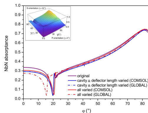
Figure 2. NbN absorbance as a function of \varphi polar angle in S-orientation ( \gamma=90^\circ ) of NCAI-SNSPD designs: reference (solid gray line), partially (COMSOL/GLOBAL: solid/dash dot blue lines) and completely (COMSOL / GLOBAL: solid/dash dot red line) optimized. Inset: polar and azimuthal angle dependent NbN absorbance of NCAI-SNSPD determined by complete optimization via GLOBAL.
